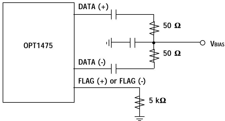
Figure 1. Interface Diagram
